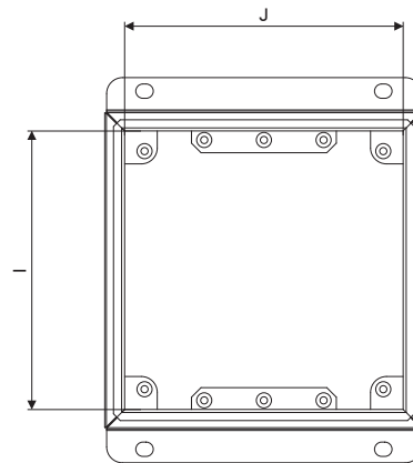
Front View Door Removed (showing internals)
